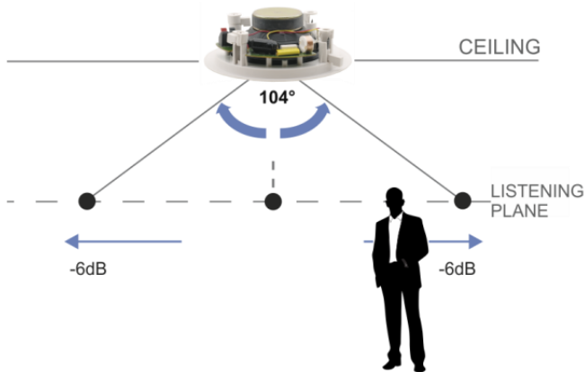
Figure 6: The Speaker Coverage Area
