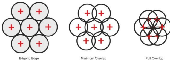
Figure 8: Hexagonal Layout
