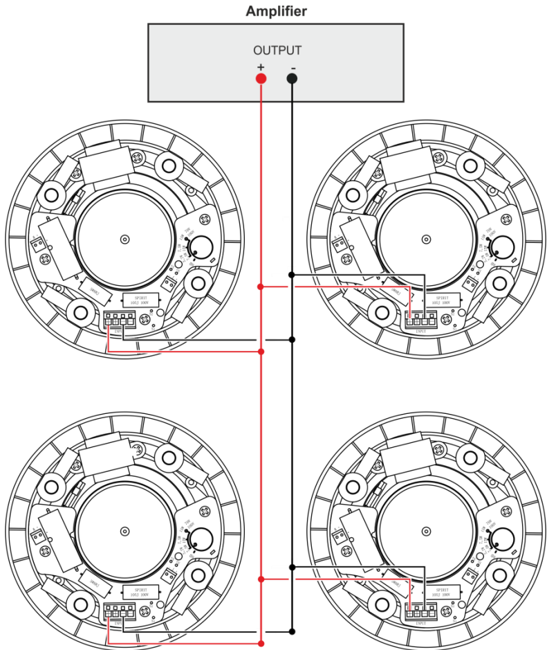
Figure 9: Square Layout Parallel Wiring
