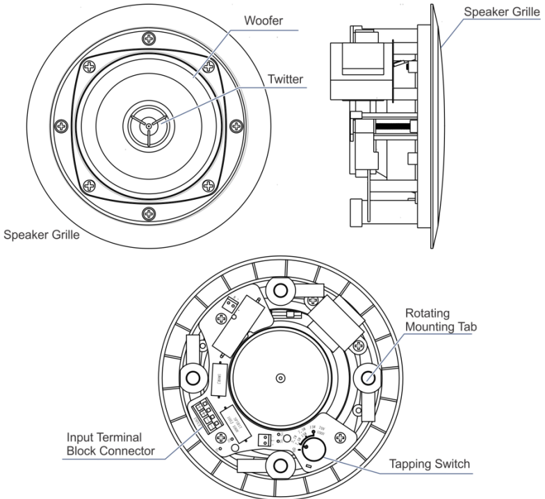
Figure 2: Galil 4-CO Open-back Ceiling Speakers
