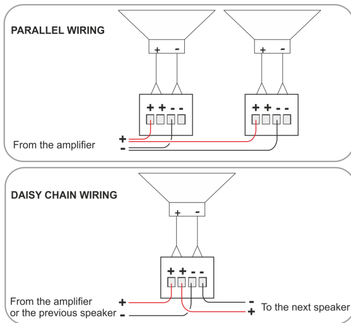
Figure 5: Open-back Ceiling Speaker Schematic Pinout Diagram
