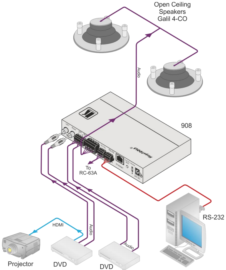
Figure 1: Open-back Ceiling Speakers in a Boardroom Setup
